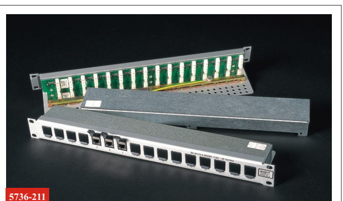
16-ports shielded patch panel with dustcovers, 1U
